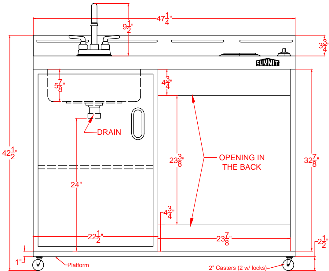
FRONT VIEW
