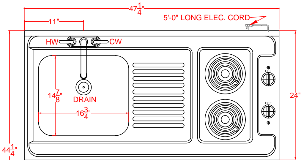
TOP VIEW
